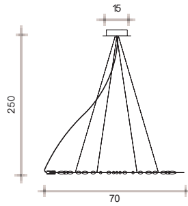
LED27W - 24V 2700°K/ 2052 lumen 3000°K/ 2160 lumen
