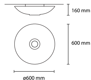
PL UFO 60 2 E27 42W ALO 1 LED 18W 1800LM 3000K
