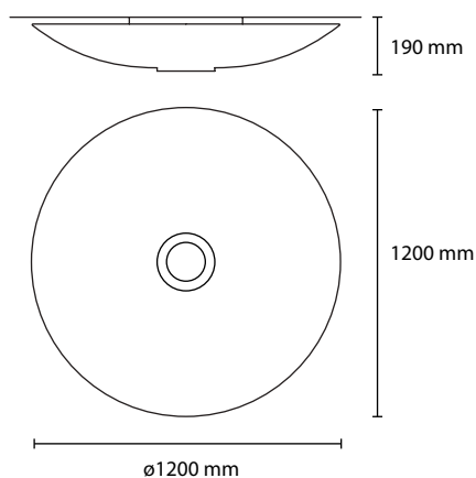
AP UFO 120 3 E27 42W ALO 1 LED 30W 2800LM 3000K
